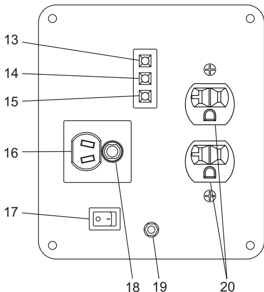
Figure 3 - Control Panel
